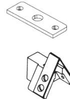
B024A130/N Blade Scraper Bracket with Cleaners (Nyleen)
