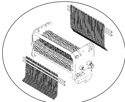
B320A Cradle Assembly - Complete Cradle, Knife Shaft Assemblies, Combs and Lock Lever
