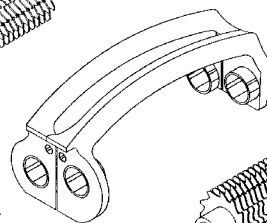
HT116F Blade Shaft Assembly -Front
