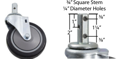
WH757 .....Swivel Caster with Square Stem
