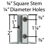
WH757 .....Swivel Caster with Square Stem
